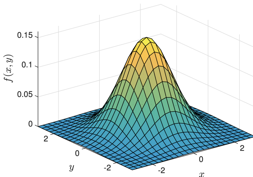
Figure 3: The joint density function f_{X,Y}(x, y) = \frac{1}{2\pi} e^{-(x^2+y^2)/2} is rotationally symmetric.
